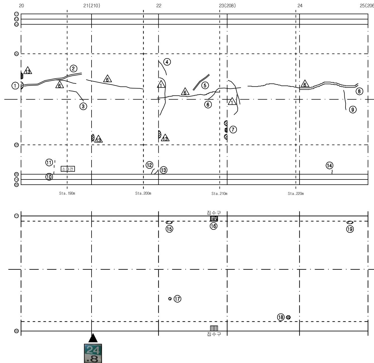
SECTION
